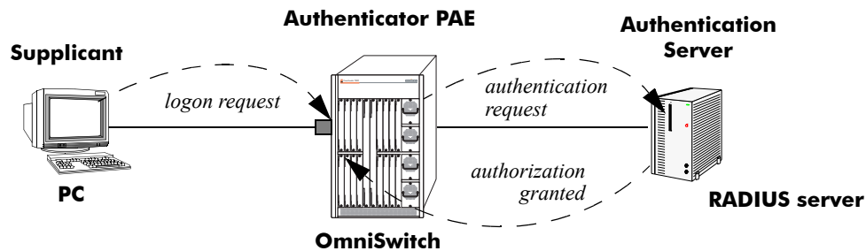
802.1X Components
