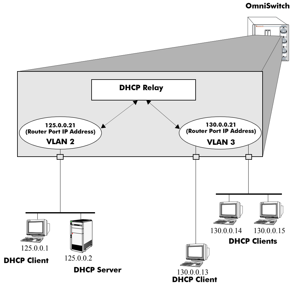
DHCP Clients in Two VLANs
